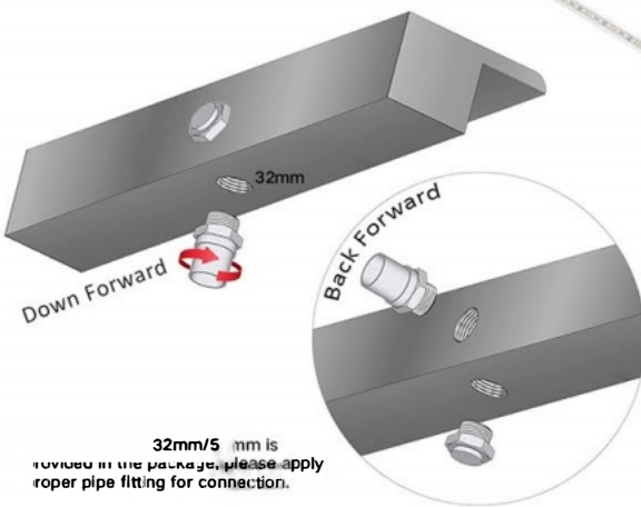
Either direction for plumbing
