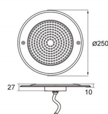
MODEL:JKD-UT250-2SP
