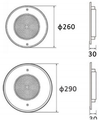
MODEL:JKD-YC260-SP JKD-YC290-SP
