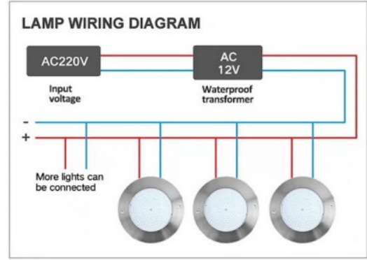
MODEL:JKD-YC260-SP JKD-YC290-SP
