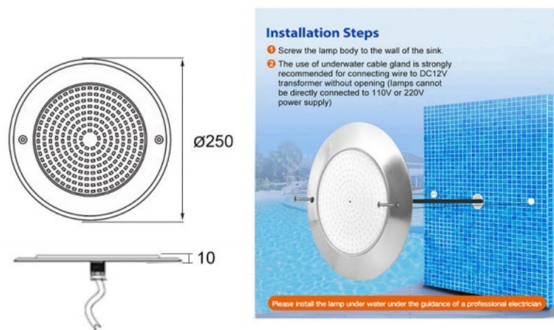
MODEL:JKD-UT250-SP
