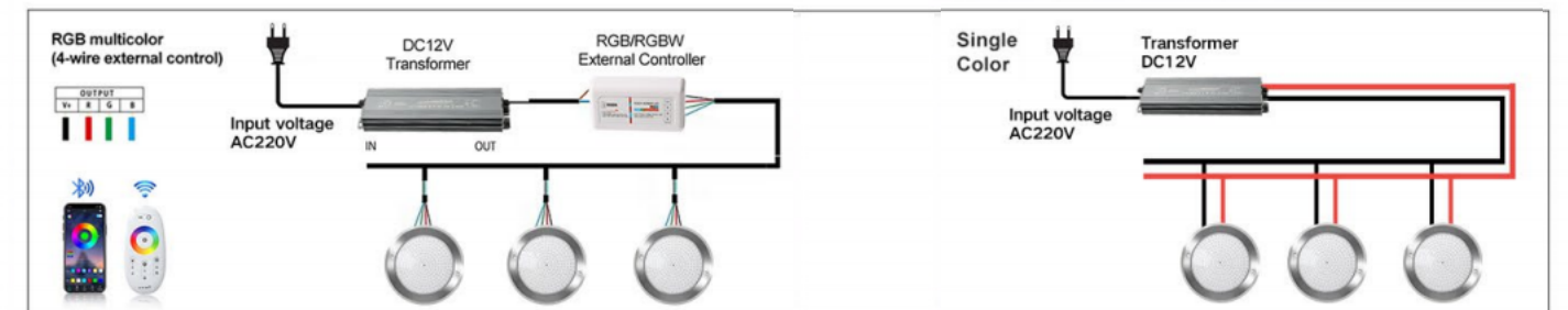
MODEL:JKD-UT230-3SP
