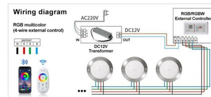
MODEL:JKD-UT230-SP
