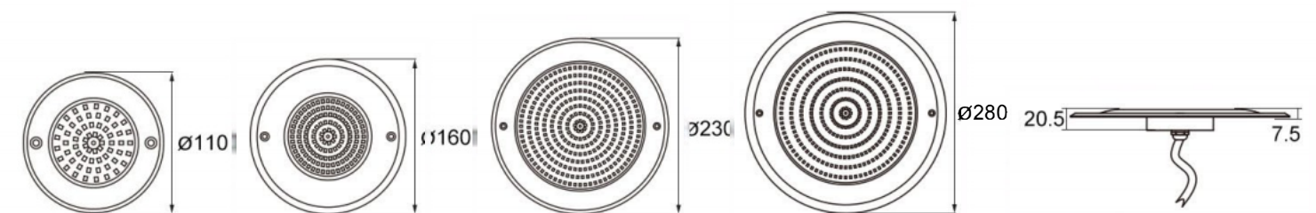
MODEL:JKD-UT230-2SP
