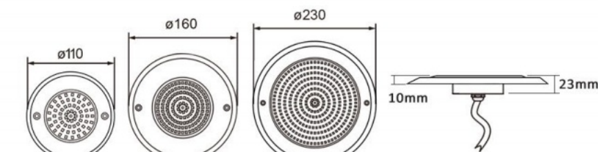
MODEL:JKD-UT230-4SP
